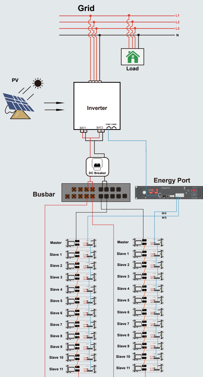
Scheme 2: 2P12S
